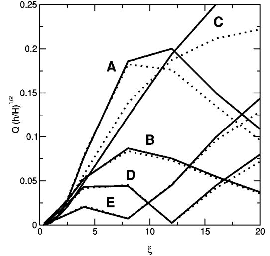
FIG. 7. Normalized separation quality Q \sqrt{h/H} vs \xi , where \xi corresponds to the force on the first species and \xi_2 = \lambda \xi , with \lambda = 2 in this plot. Full lines, results of Monte Carlo simulation; dotted lines: Master equation. The difference is due to the larger values for the diffusion tensor component \bar{D}_{xx} at high force \xi yielded by the master equation. The location of the optimum does not change much. See discussion in the text.
