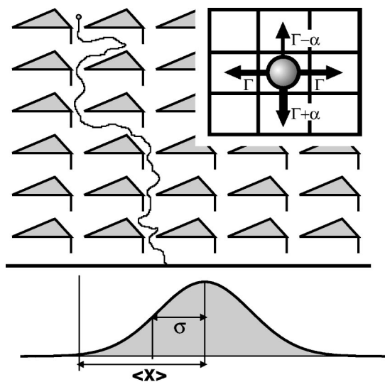
FIG. 1. The model situation: A particle diffusing and drifting through a periodic array of obstacles. When it has reached the final row of the array, its horizontal deflection is registered, which leads to a Gaussian distribution for an ensemble of many particles (after coarse graining over several obstacles). The inset shows the transition rates used in the Monte Carlo simulations on a lattice.
