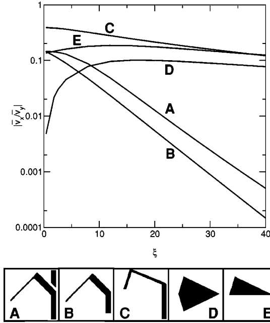
FIG. 6. Slope \langle x \rangle / H = \bar{v}_x / \bar{v}_y plotted vs \xi . The obstacle shapes are shown at the bottom of the plot and are discussed in the text. A refers to the obstacle shape shown in Fig. 3.
