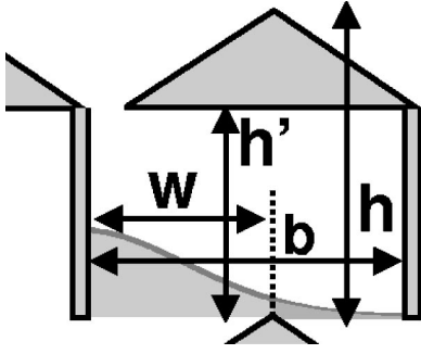
FIG. 2. Parameters entering the analytical estimate of the macroscopic drift velocity. The spreading Gaussian distribution is cut into two halves (see text).
