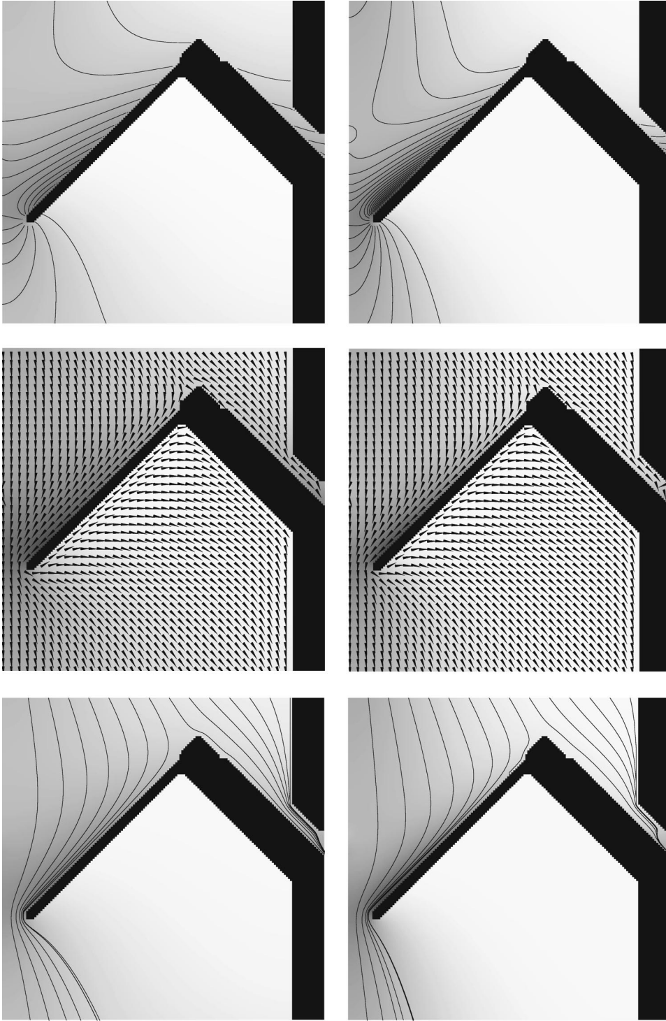
FIG. 3. Distribution p (top), velocity direction field \hat{v} (middle), and “streamlines” (bottom) for low and high force (left and right columns). The strength of the force \xi=12 for the left column and \xi=24 for the right column, with the microscopic drift pointing downward. Darker shading signifies increased p . Contour lines for p have been chosen at the same (equidistant) values for the two pictures at the top. Note that the streamlines serve to visualize the direction of the current density, while the real motion of a single particle is governed by drift and diffusion. The “velocity direction” is the normalized current density vector field. Note the stronger pileup in density at the left “roof” of the obstacle for the stronger force, as well as the distortion of streamlines there and in the narrow channel at the right of the pictures. The lattice shown here consists of 160 \times 160 sites.
