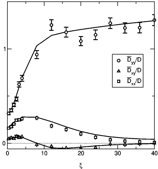
FIG. 5. Components of macroscopic diffusion tensor vs \xi for the obstacle of Fig. 3. Circles, \bar{D}_{yy}/D ; squares, \bar{D}_{xx}/D ; triangles, \bar{D}_{xy}/D . Symbols show results of the Monte Carlo simulation, lines show those of the master equation. We attribute the deviation at higher values of \xi (and, therefore, \alpha/\Gamma ) to effects of the finite grid resolution.
