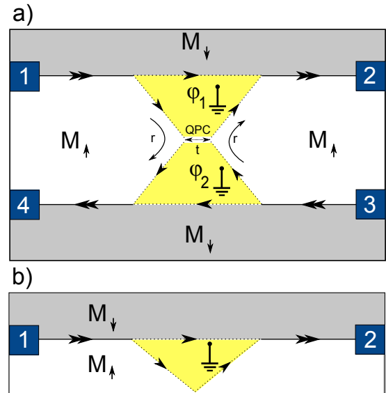
FIG. 2: (a) Modified Hanbury Brown-Twiss interferometer. Majorana excitations will propagate along the boundaries of the two triangular superconducting structures with phases \varphi_1 , \varphi_2 . An additional short gapped channel appears at the domain wall between the two superconducting regions, forming a quantum point contact characterized by reflection and transmission amplitudes r , t . The setup is similar to the one proposed in Ref. 7. (b) In the fully transmissive case, t = 1 , r = 0 , the device splits into two separate Mach-Zehnder interferometers, one of which is shown here.
