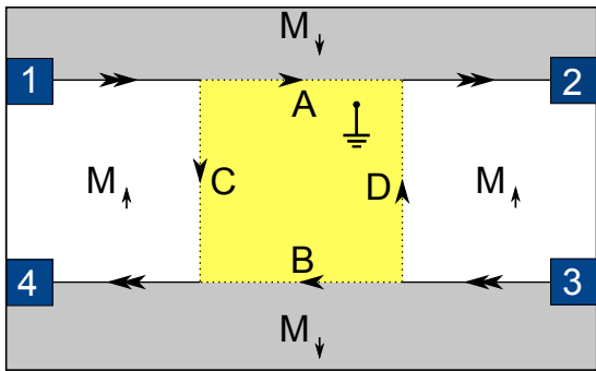
FIG. 1: Hanbury Brown-Twiss type interferometer. A grounded superconductor surrounded by four magnetic domains is placed on the surface of a three-dimensional topological insulator. The terminals 1, 2, 3, and 4 are connected to the outside circuit and biased at potentials V_1, \dots, V_4 respectively. The magnetizations are chosen such that Dirac electron states at leads 1, 2, 3, and 4 exist and propagate in the direction of the double arrows. Electrons and holes can enter the interferometer at leads 1 and 3, Majorana fermions propagate along the arms A, B, C, and D in the direction of the single arrows and electrons and holes leave through leads 2 and 4. A magnetic flux in the form of n_v vortices threading the superconductor will control the phase difference between the arms of the interferometer.
