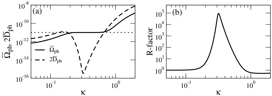
FIGURE 2. The same as Fig. 1 for the driving strength \varepsilon_0 = 5 .
